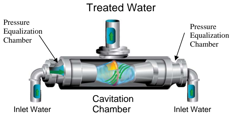
Figure 3. Diagram of the Hydrodynamic Cavitation Equipment
