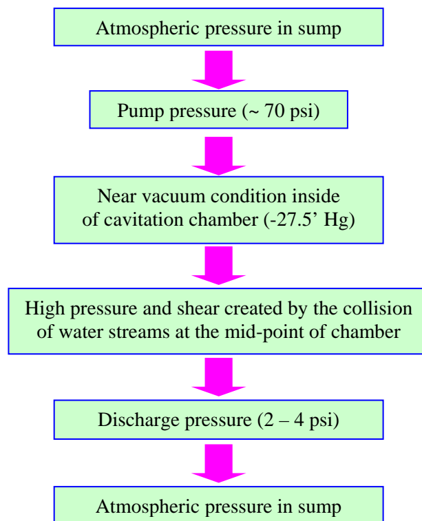
Figure 4. Changes in Pressure of Water Passing CHC Unit
